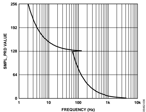
Figure 36. SMPL_PRD Values vs. Sample Frequency
